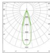
30° PC Lens
