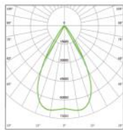
60° PC Lens
