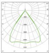
90° PC Lens
